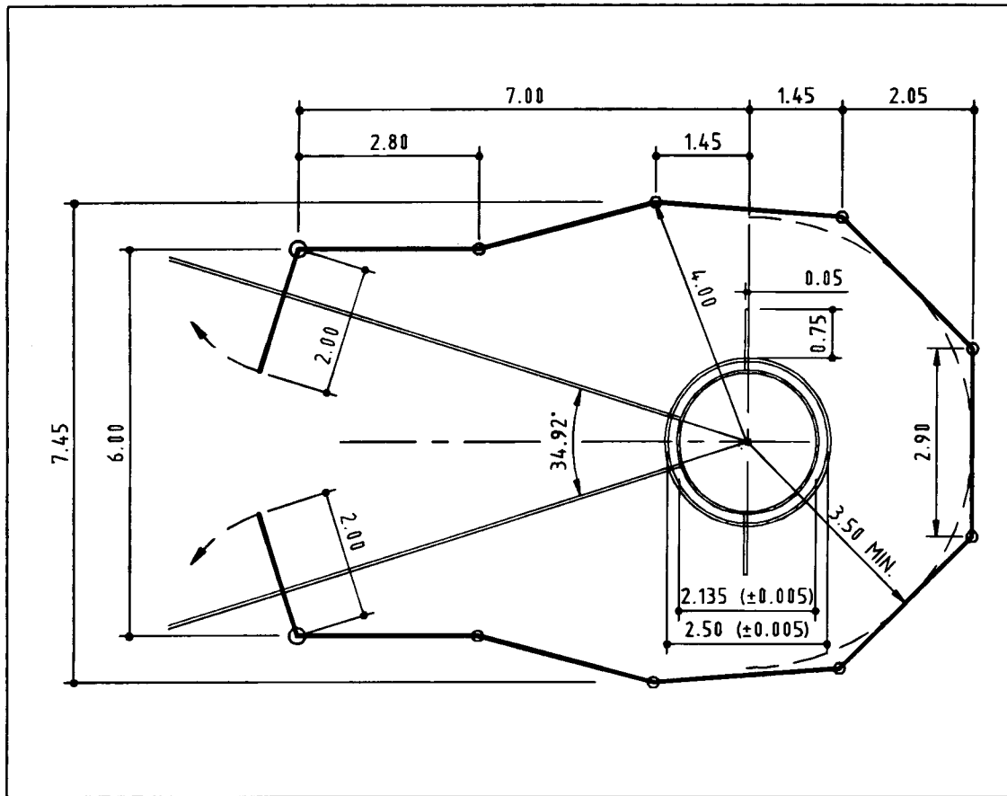
Combined discus and hammer throwing cage No 1 with concentric circles (Dimensions in m)
